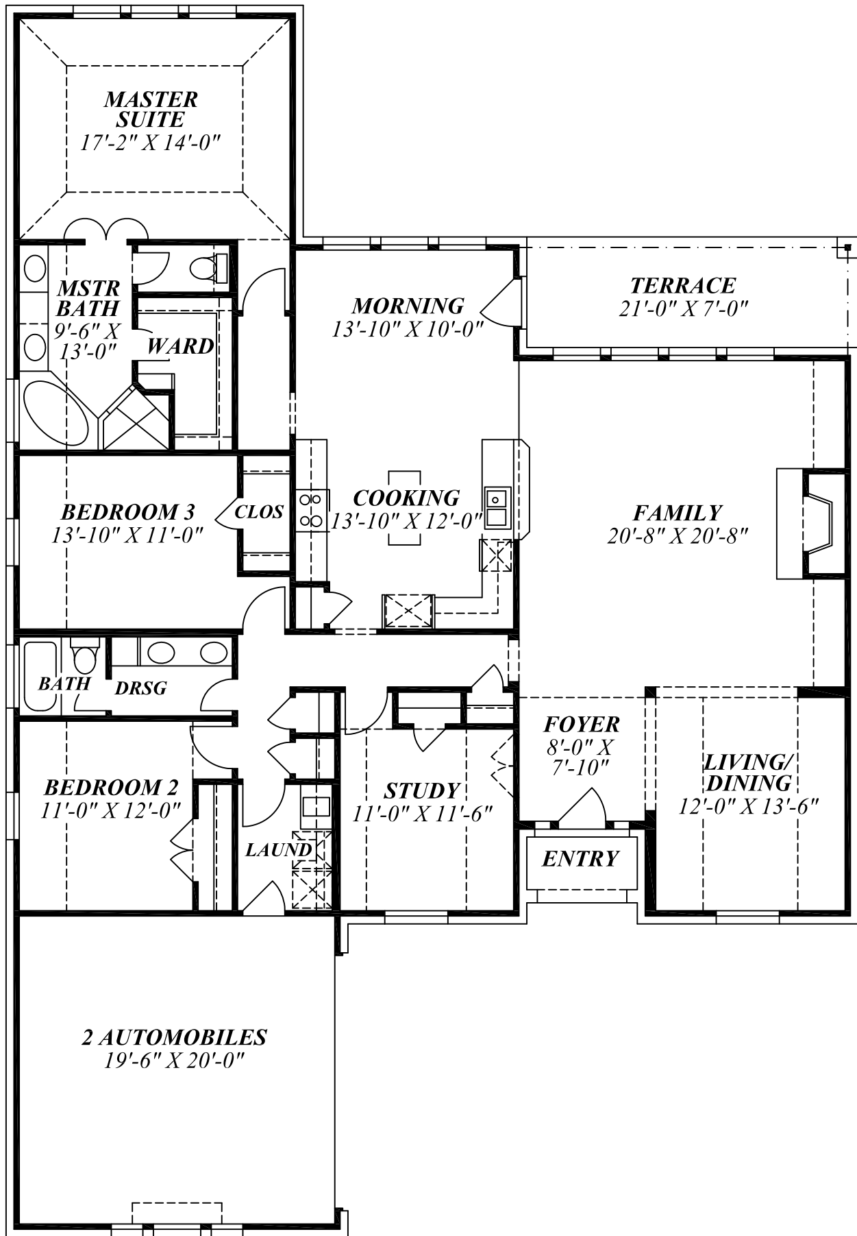
FLOOR PLAN
