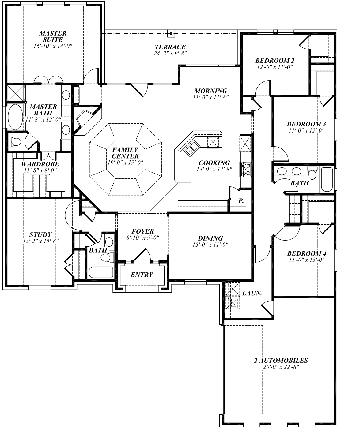
FLOOR PLAN
