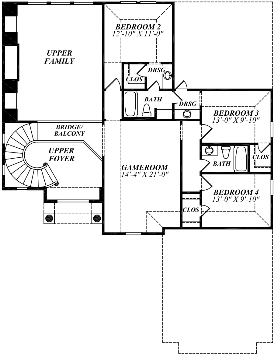
UPPER LEVEL FLOOR PLAN
