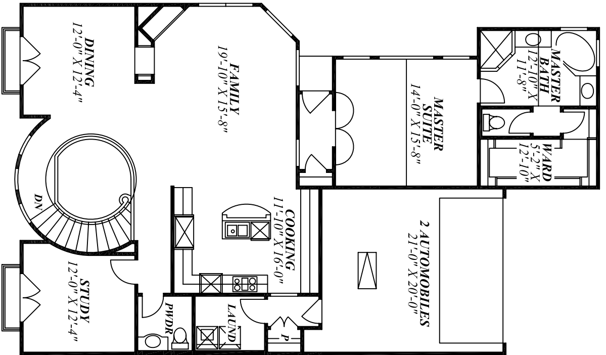
MAIN LEVEL FLOOR PLAN
