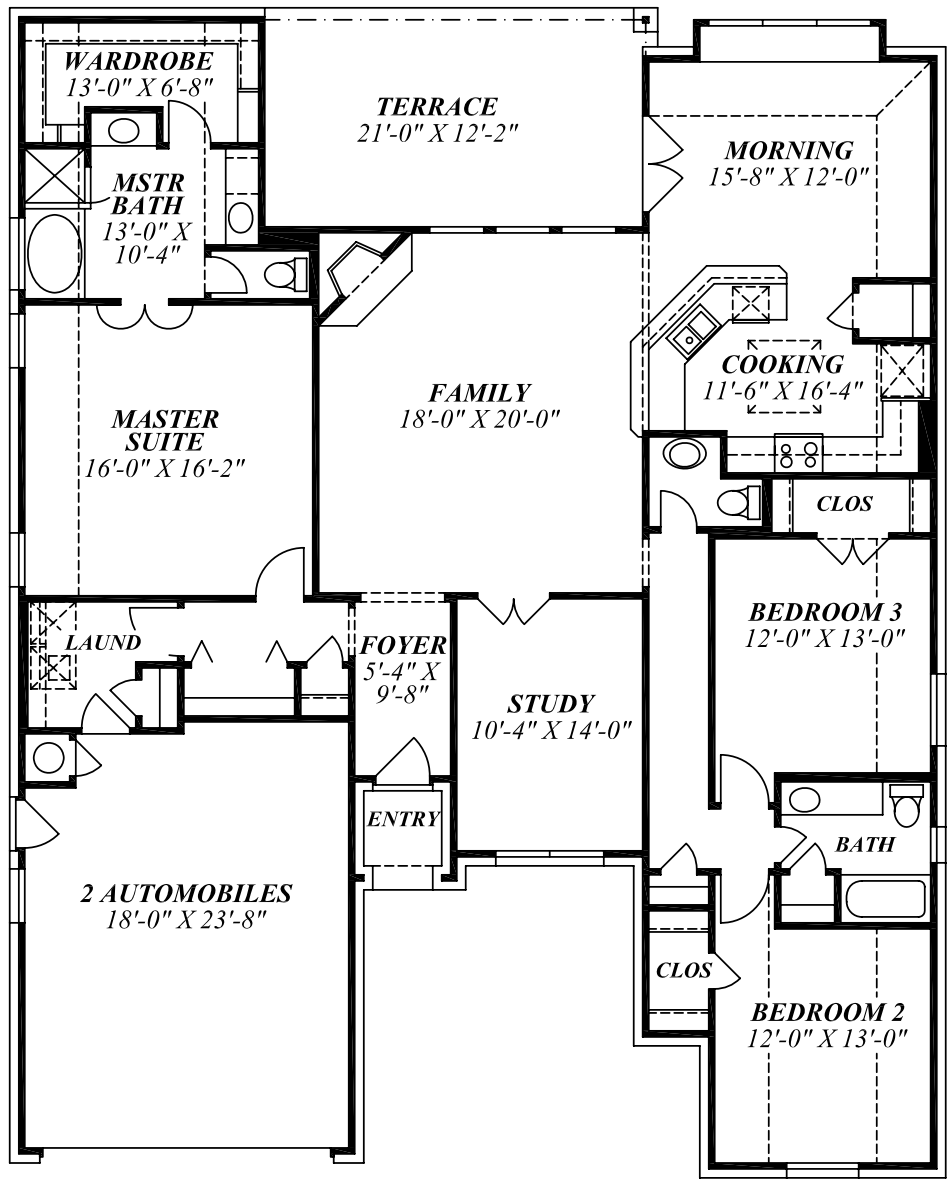
FLOOR PLAN
