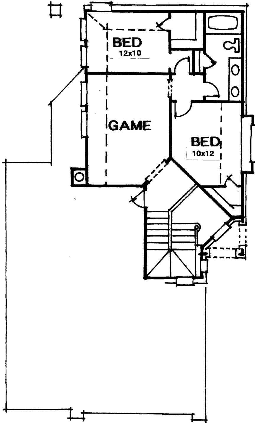
SECOND FLOOR FC-2000
