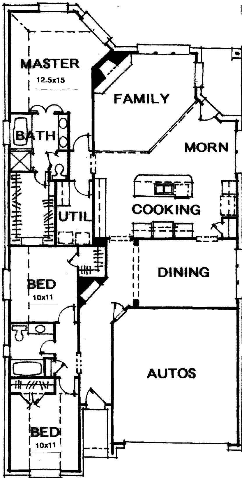
FLOOR PLAN FC-1800
