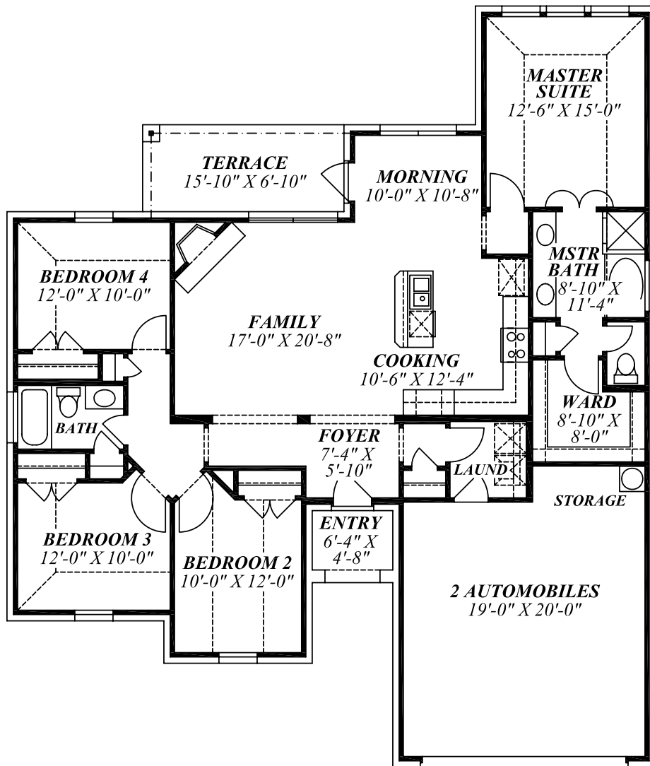
FLOOR PLAN
