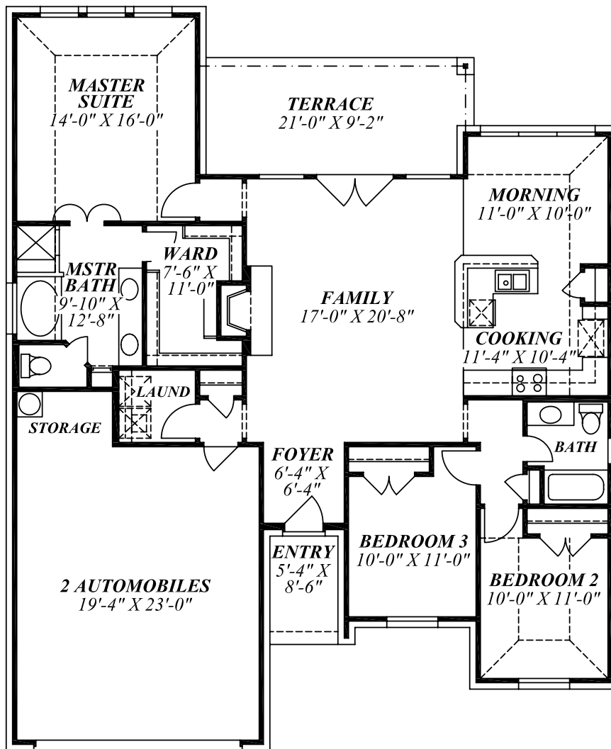
FLOOR PLAN
